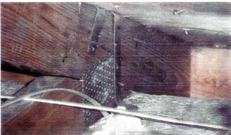
Single wrap with at least 2 nails on the embedded side and 1 nail on the wrapped side
