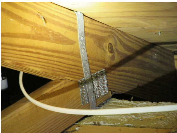
Single wrap Roof To Wall Attachment
