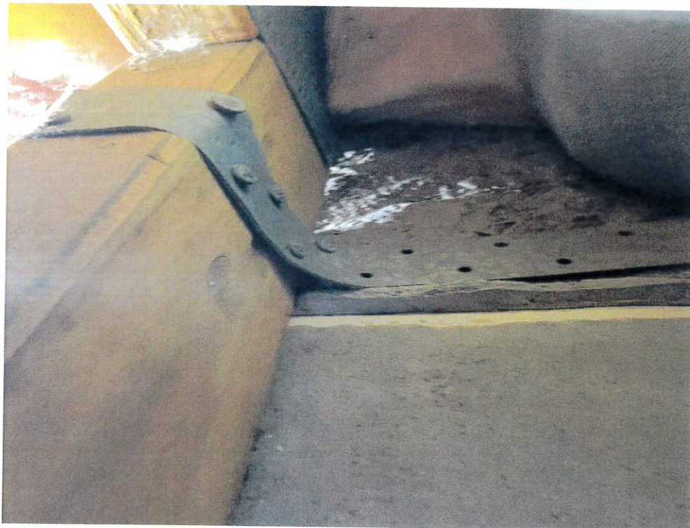
Figure 6 - Roof to Wall Attachment
