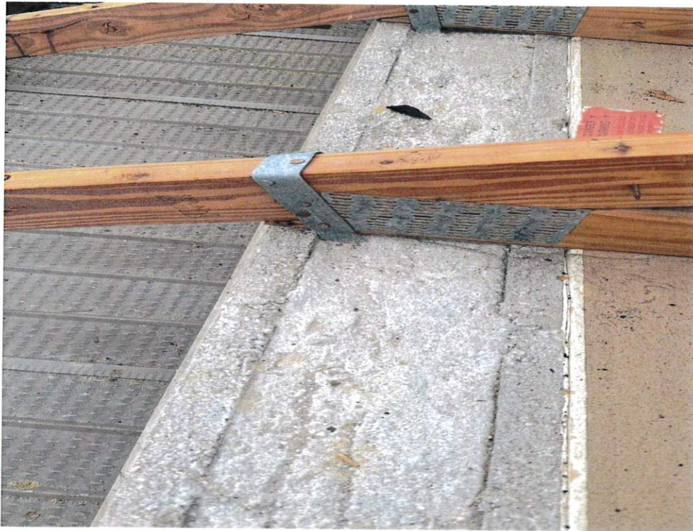
Figure 5 – Roof to Wall Attachment
